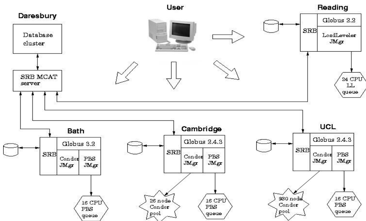
Figure 1: Schematic representation of the compute and data resources within the eMinerals Minigrid Infrastructure.
