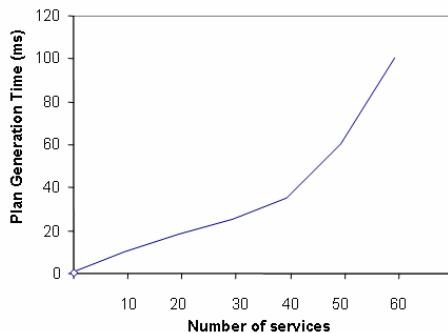
Fig. 3. Plan Generation Times.
