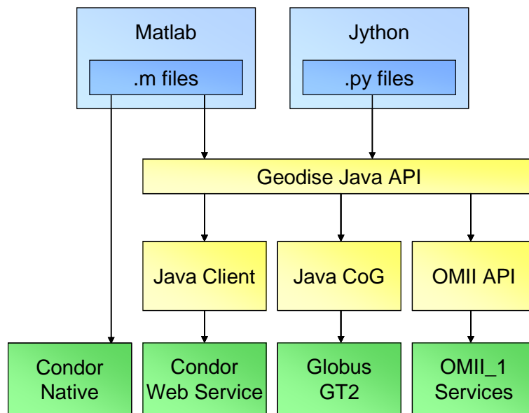
Figure 2 GeodiseLab Compute Toolboxes
