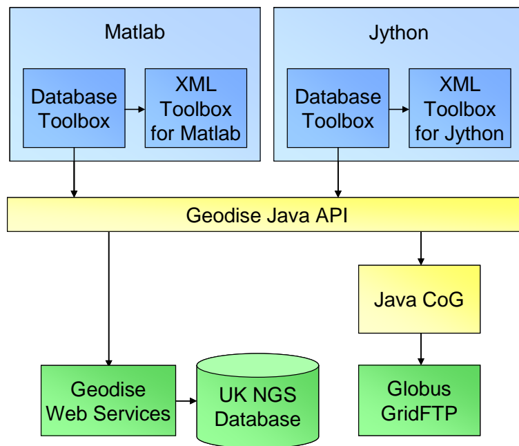
Figure 3 Geodise Database and XML Toolboxes
