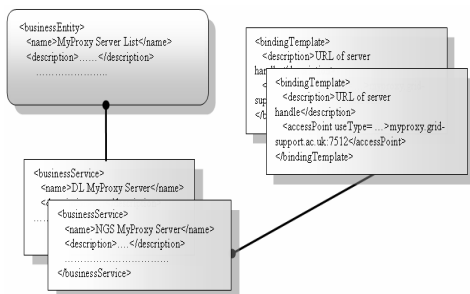
Figure 3: UDDI data model
